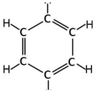
HYDROCARBON
